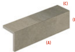
PROFILE* 6x24x0.8 cm | GJ33 (A: 24 cm / B: 6 cm / C: 6 cm)
